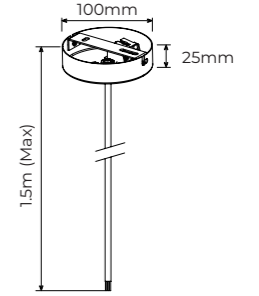
ACC-DB160-(DA/D0)-BK(WT)-0200 Round ceiling plate
